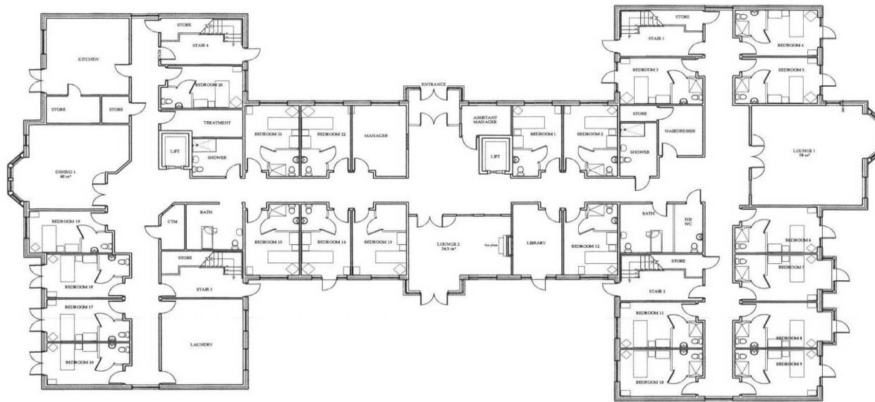
L [0] 01 Level 1 Plan Total Floor Area - 1179m/sq
